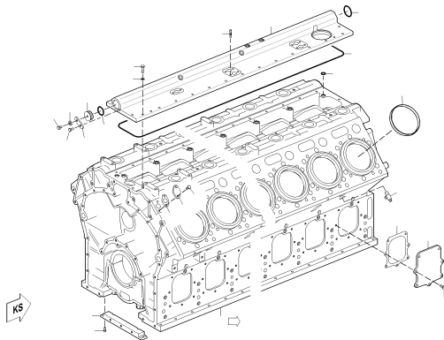
CRANKCASE X00026310
